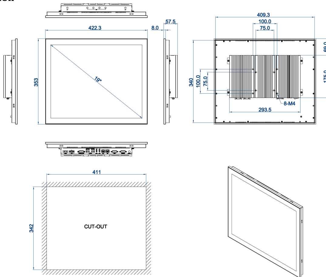
DIMENSIONAL DRAWING:TPC-DCS190
